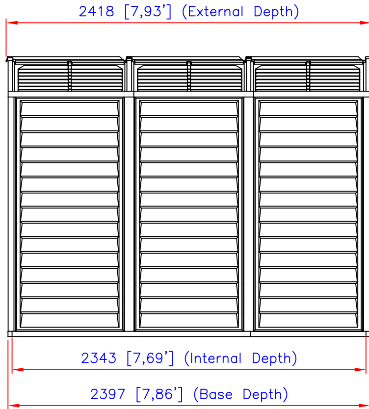
Side View
